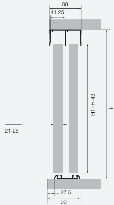
21-25mm Door thickness
